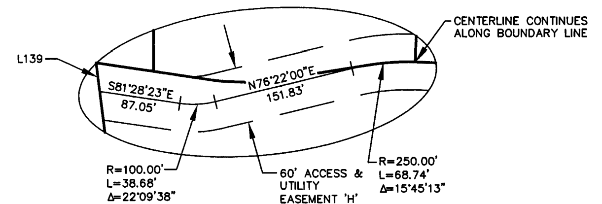
DETAIL 'A' SCALE: 1" = 100'
